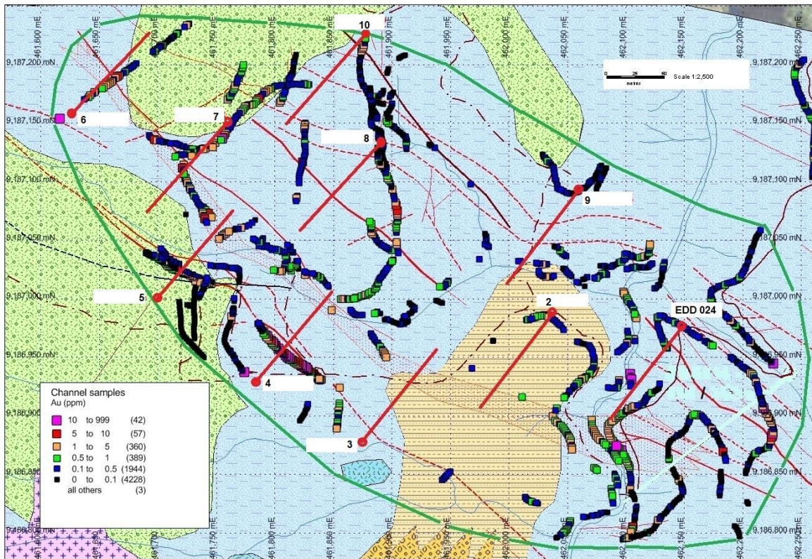
Figure 3: Enterprise – Karuka stockwork zone with position of EDD 024, EDD 025 (shown as 2 above) and proposed remaining drill pattern.
